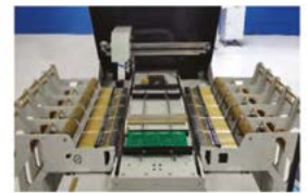
12 Lane, 88MM Bank Feeders
